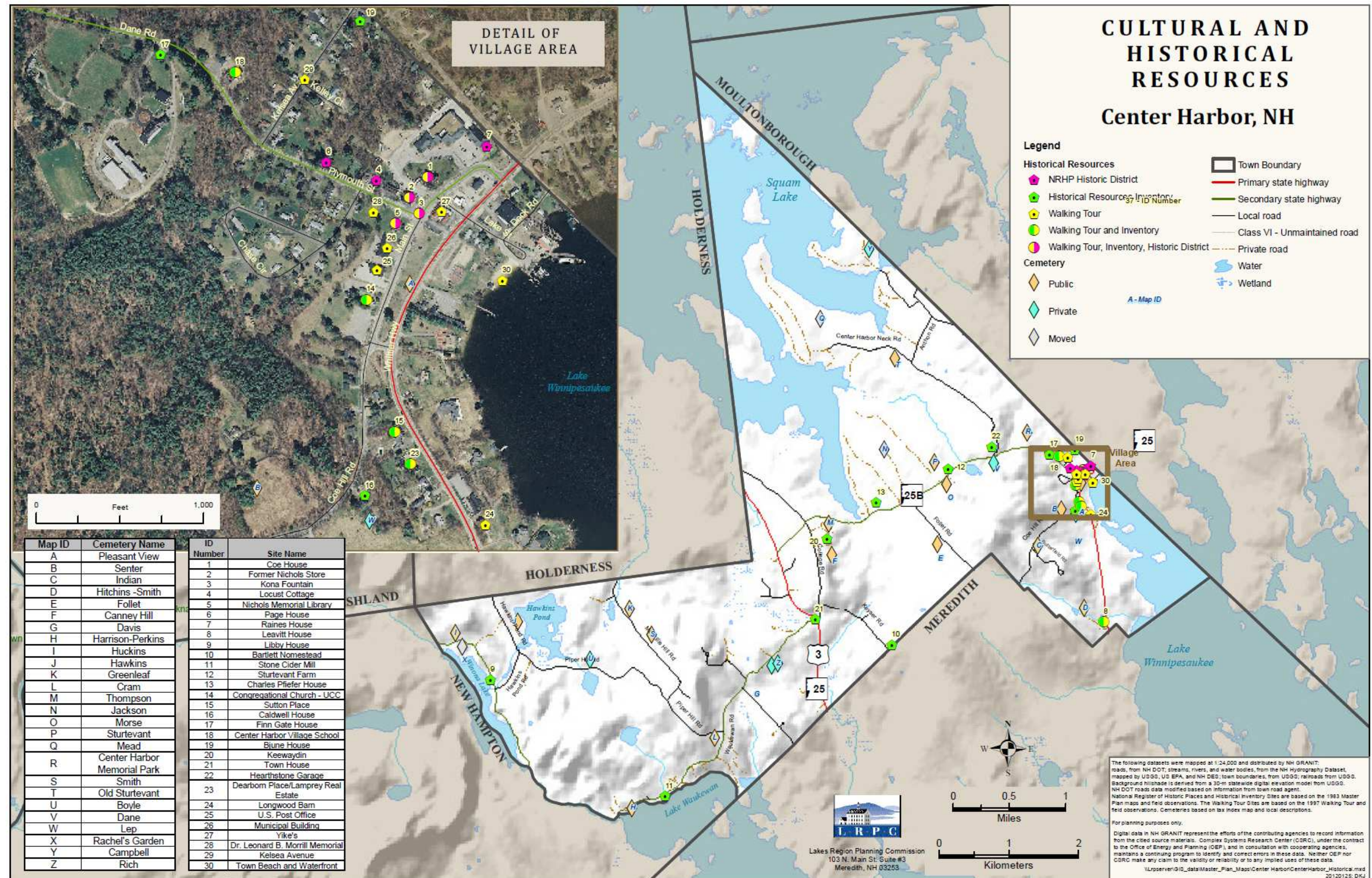
Map 7-1: Center Harbor Cultural and Historical Resources
